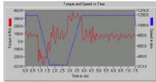
Fig. 2: Speed and Torque vs. time.
