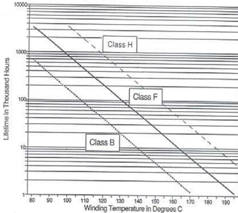
Fig 1: Winding Temperature vs. Lifetime for Insulation Class B, F, & H
